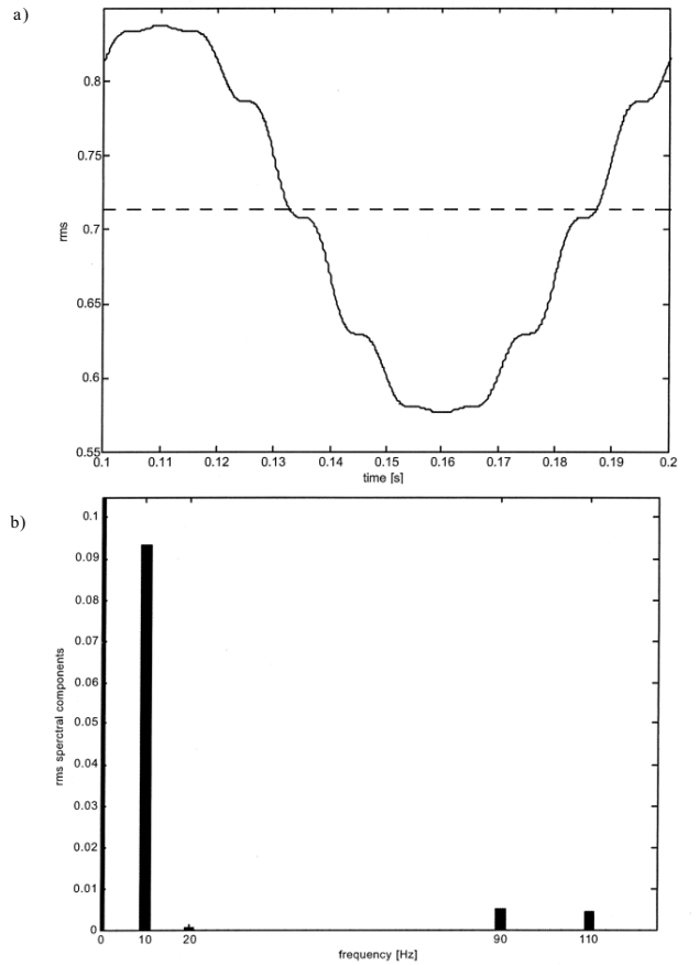
Fig. 5. Case-study 2: a) RMS value calculated over a 20 ms shifting window versus the time (—) and RMS value calculated from Fourier expansion over 100 ms (---); b) spectrum of curve (—)
